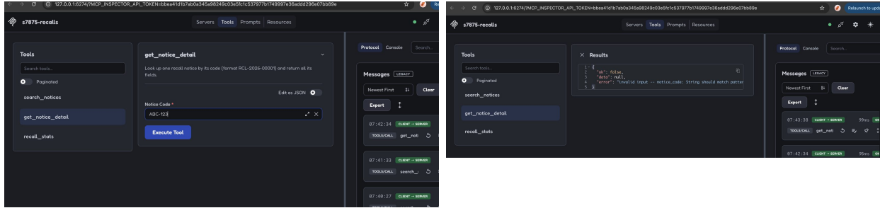
Figure 34. get_notice_detail - invalid call (ABC-123), rejected.
