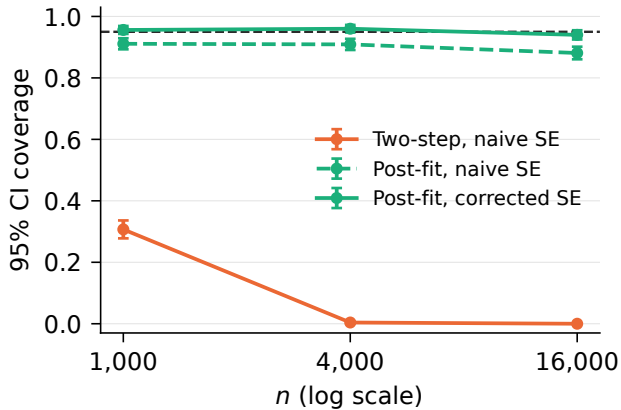
Roll-call votes (2PL IRT)
