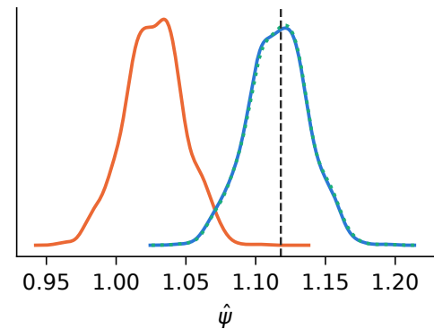
Linear-Gaussian, n=4,000
