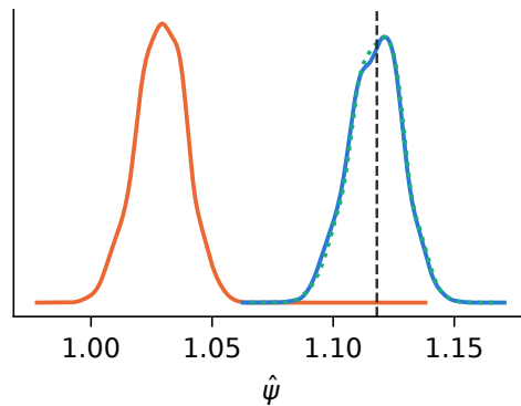
Linear-Gaussian, n=16,000
