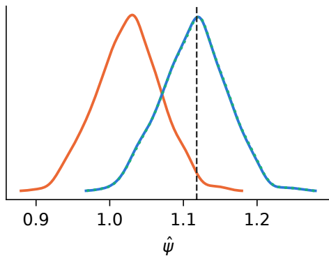
Linear-Gaussian, n=1,000
