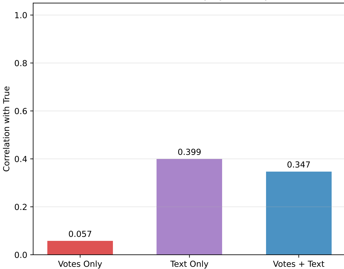
Ideal Point Recovery by Modality
