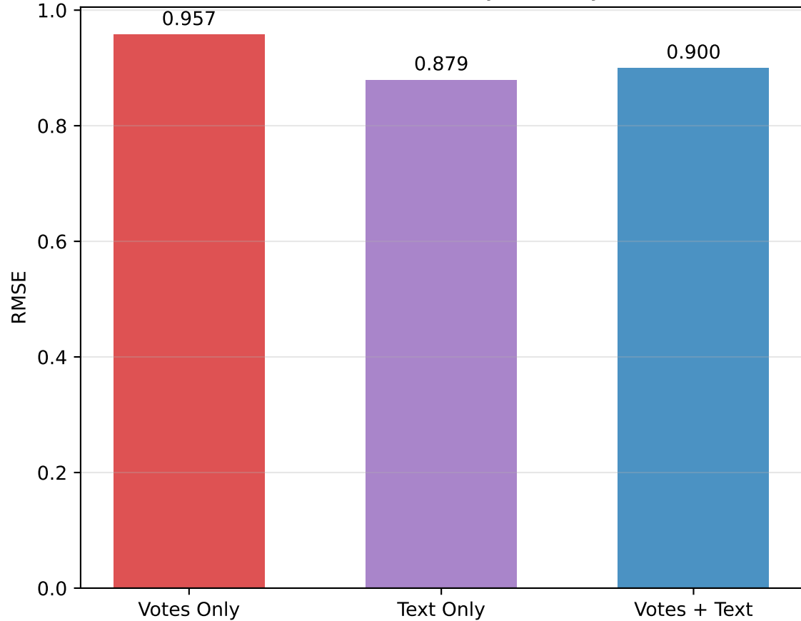
Estimation Error by Modality
