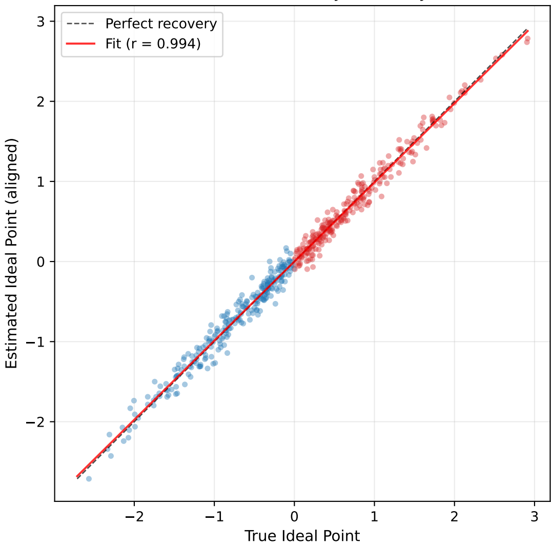
Ideal Point Recovery: Text Only
