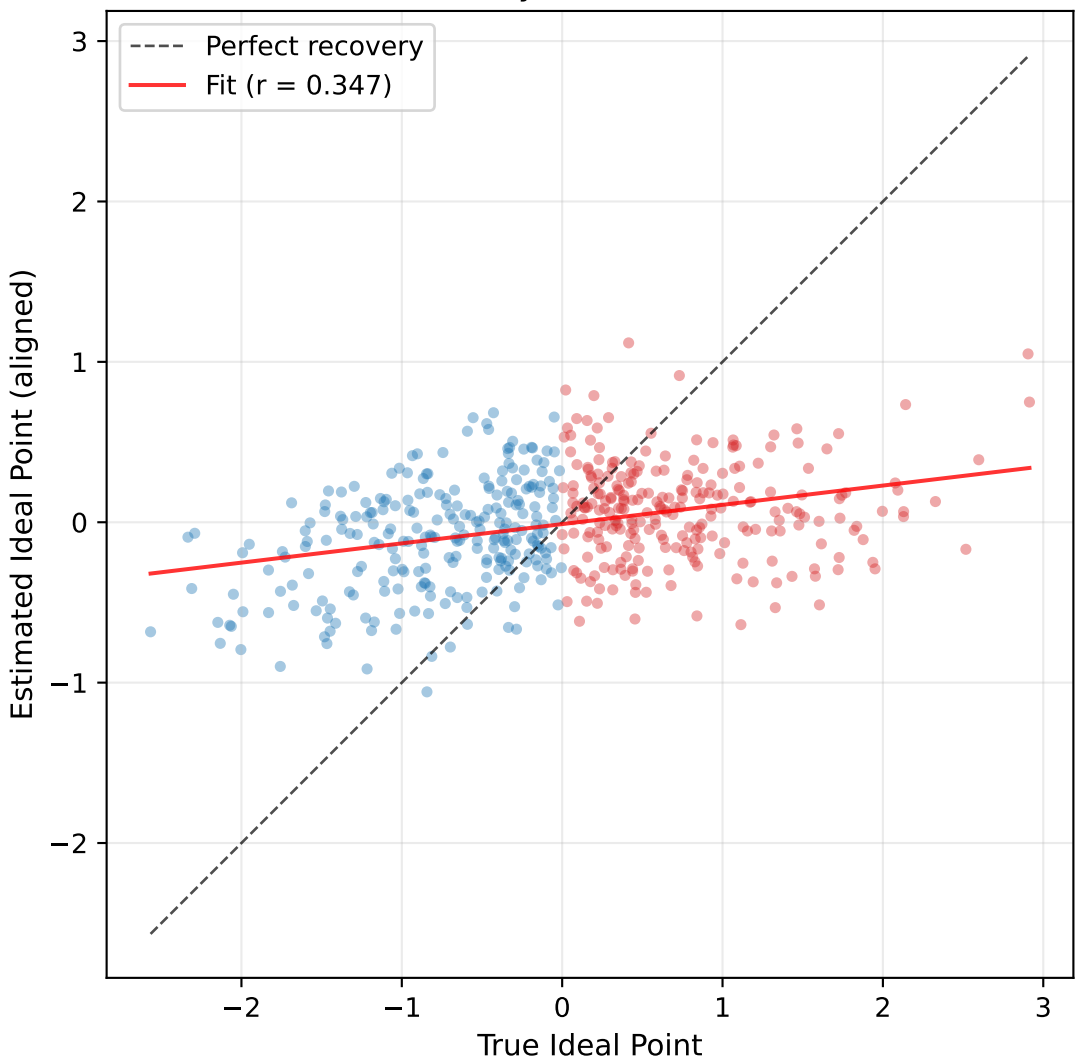
Ideal Point Recovery: Votes + Text (Multimodal)
