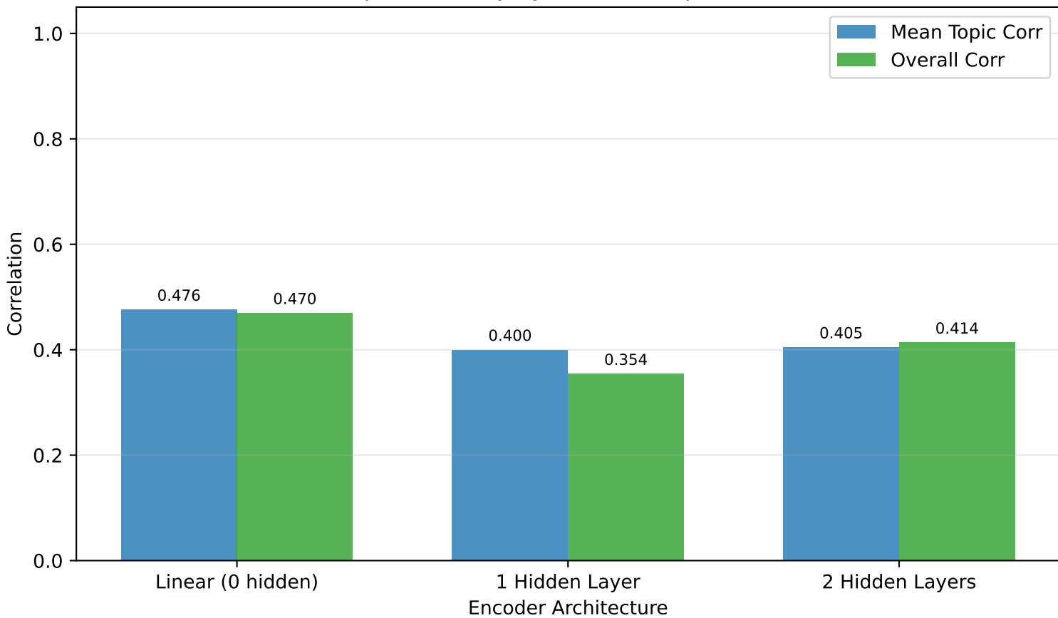
Topic Recovery by Encoder Depth (K=3)
