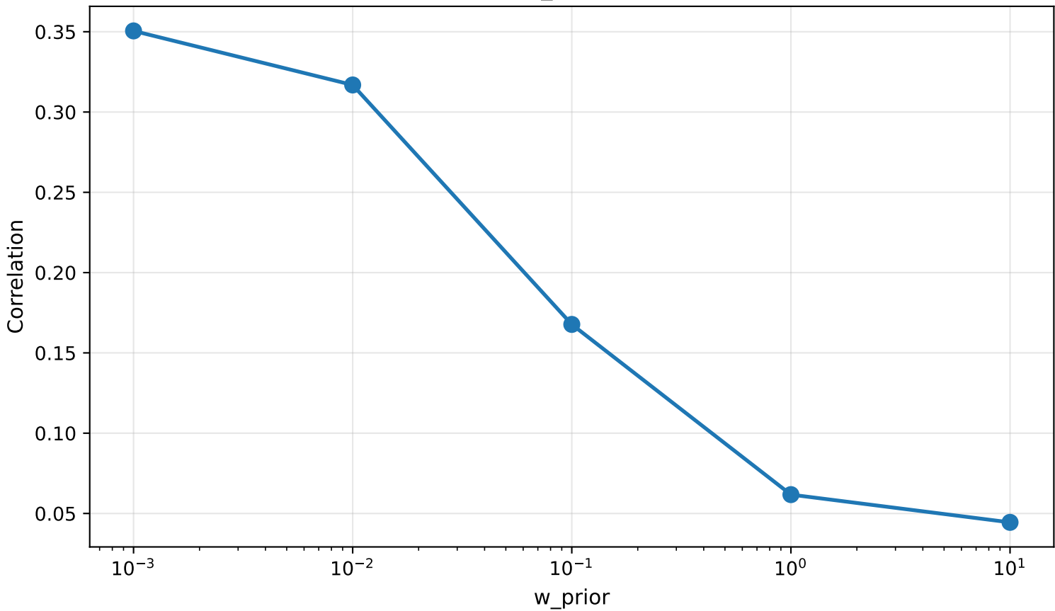
Sensitivity to w_{\text{prior}} (IdealPointNN)
