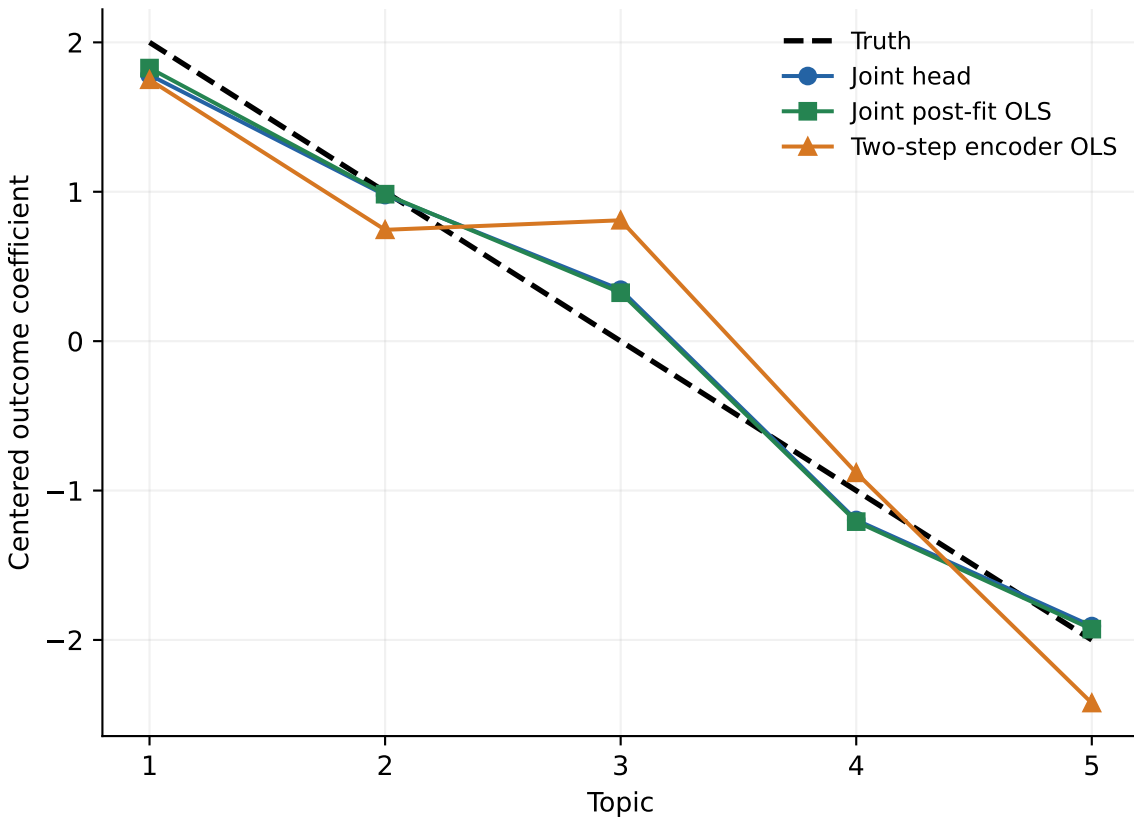
One replication: outcome coefficient recovery
