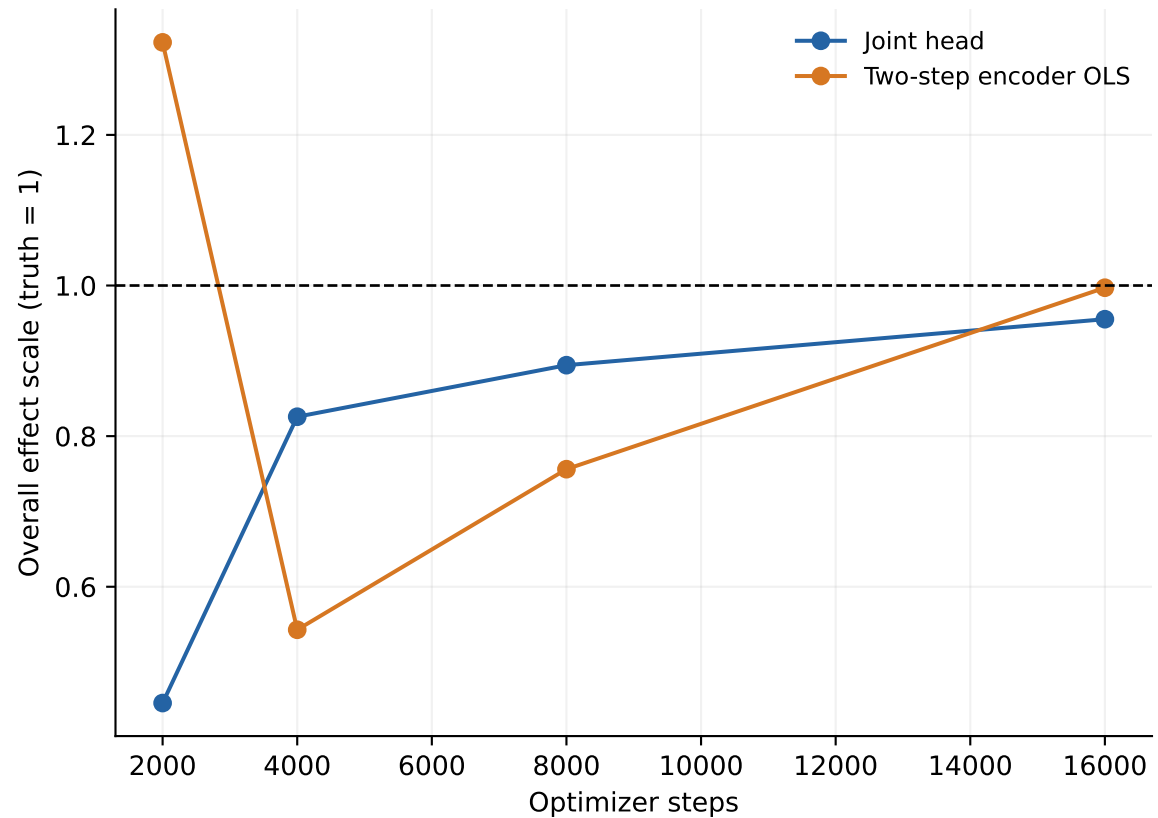
Training trajectory; all planned checkpoints
