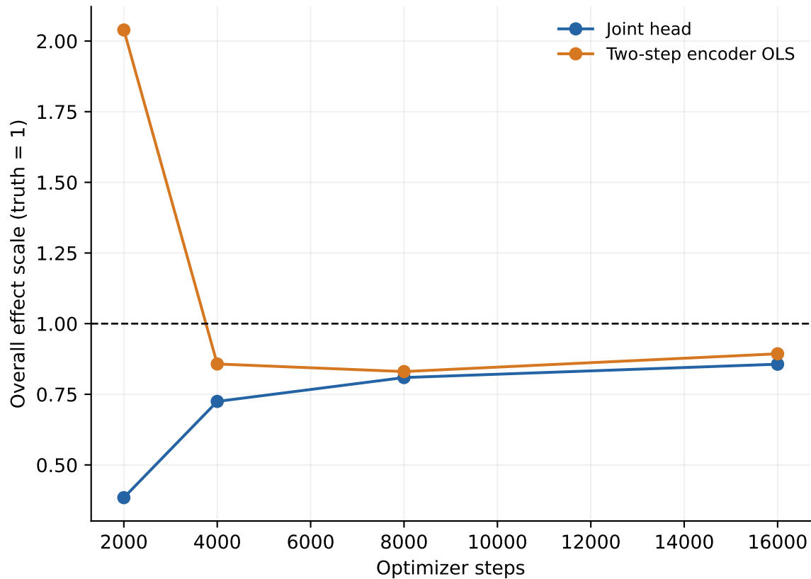
Training trajectory; all planned checkpoints
