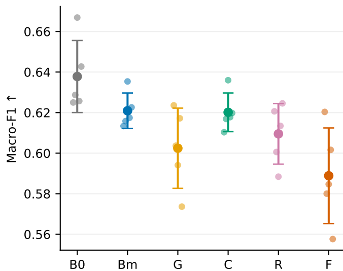
Module ablation under continuous missingness
