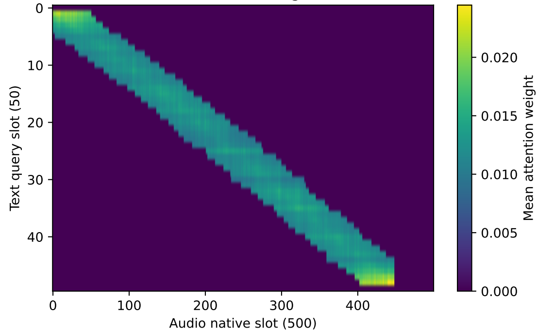
Text → Audio soft alignment
