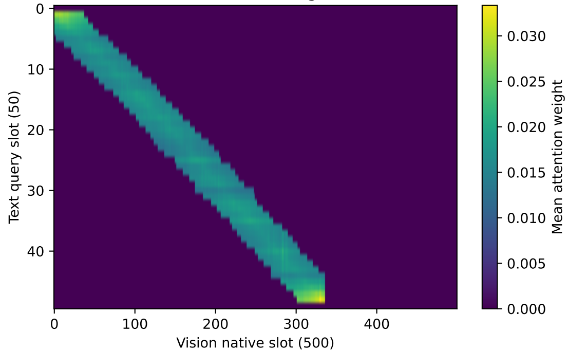
Text → Vision soft alignment
