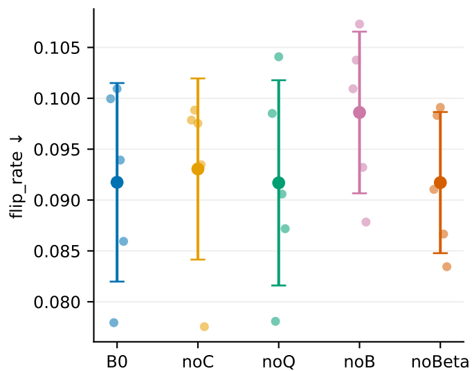
Paired full/missing prediction stability
