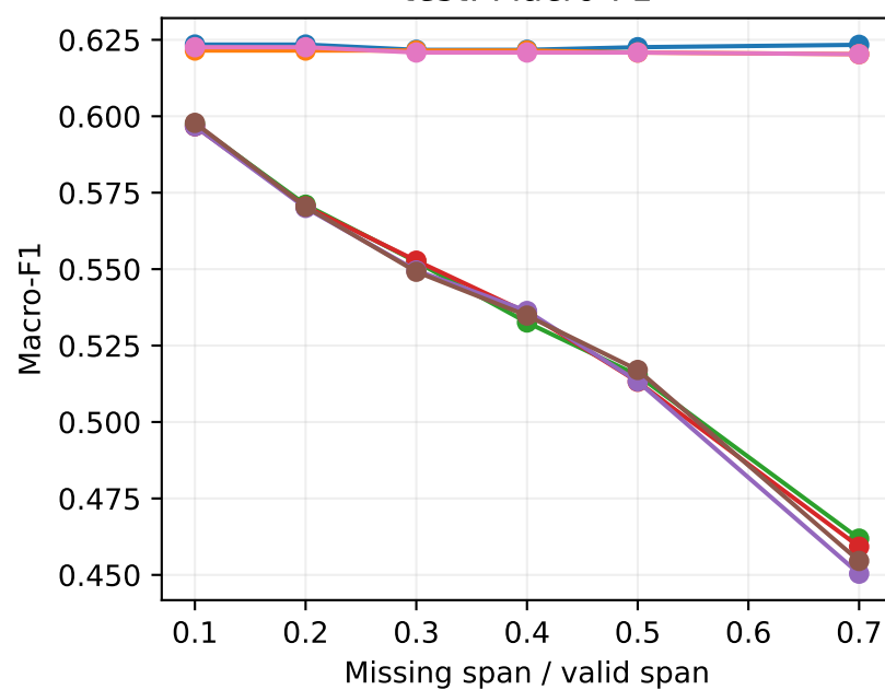
test: Macro-F1
