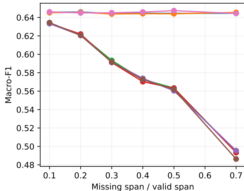
test: Macro-F1
