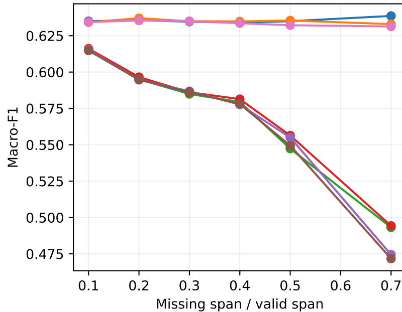
test: Macro-F1
