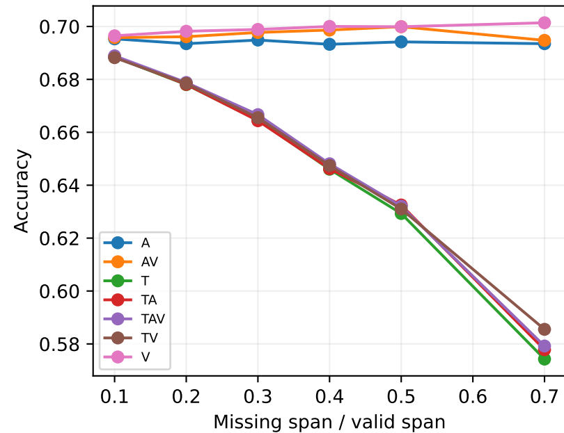
test: Accuracy
