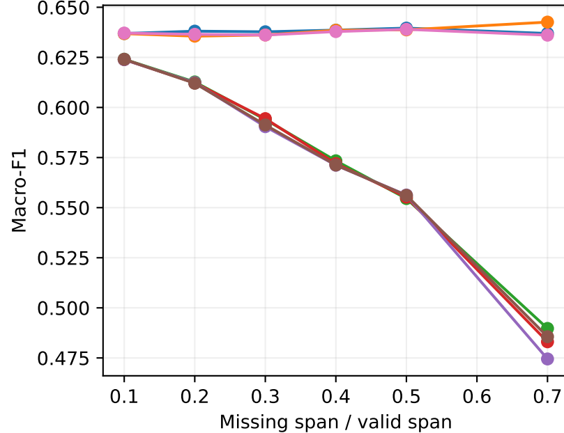
test: Macro-F1
