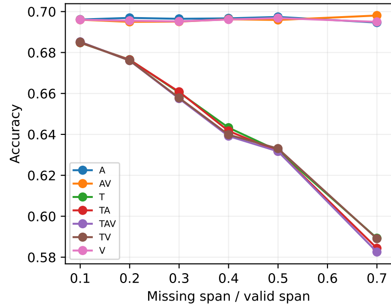
test: Accuracy
