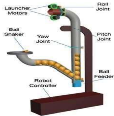
Gambar 3. mTTTbot: Multiple Style Table Tennis Trainer & Ball Launcher Robot [3].
