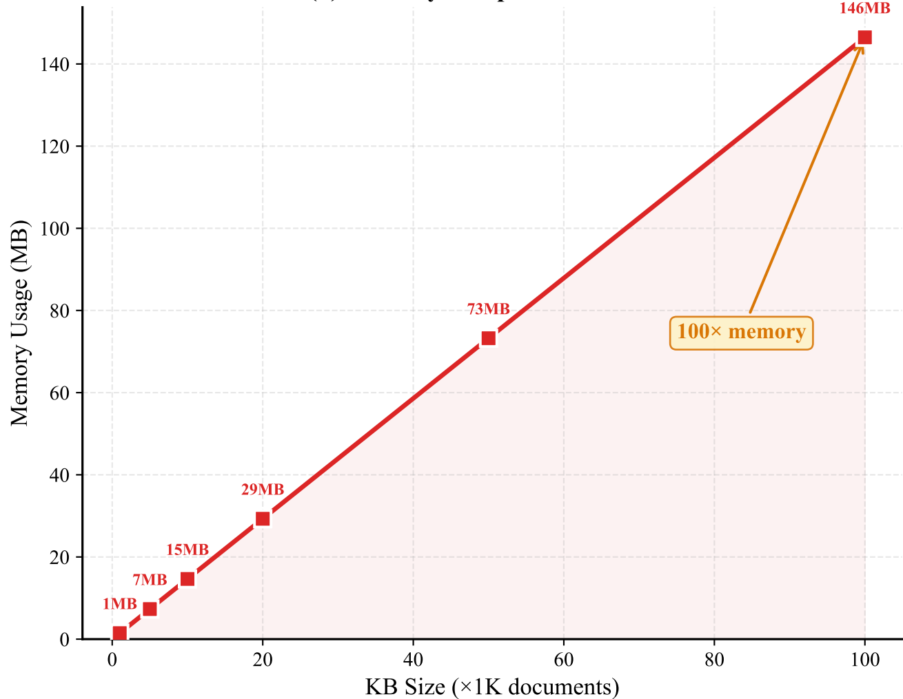
(b) Memory Footprint vs KB Size
