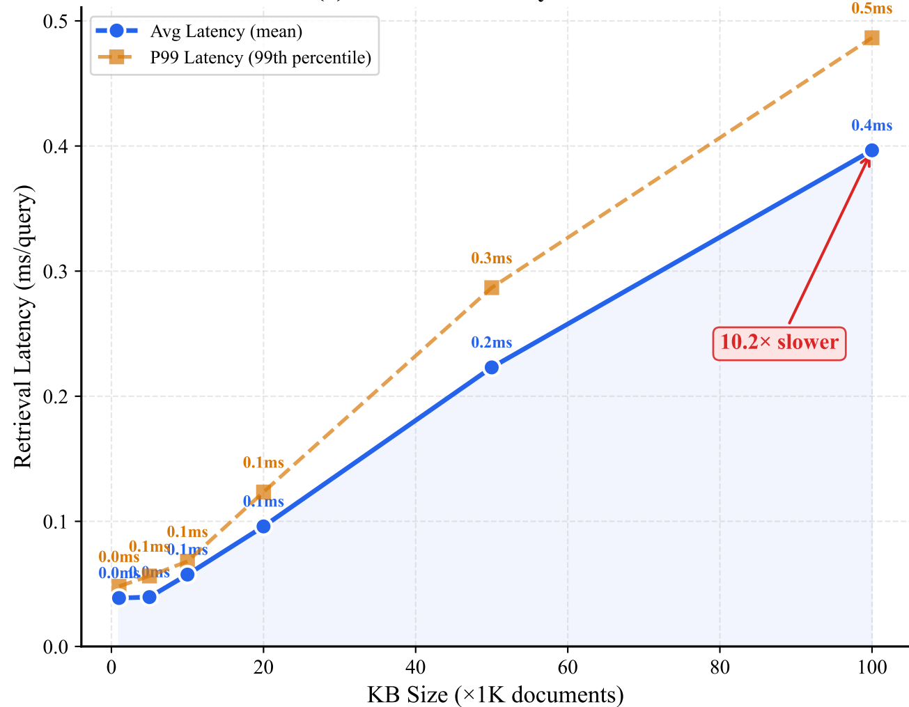
(a) Retrieval Latency vs KB Size
