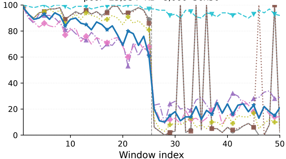
2Wiki-comparison pool=25,954 KB=8,000 50x50
