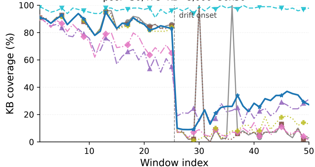
HotpotQA-comparison pool=30,478 KB=8,000 50x50
