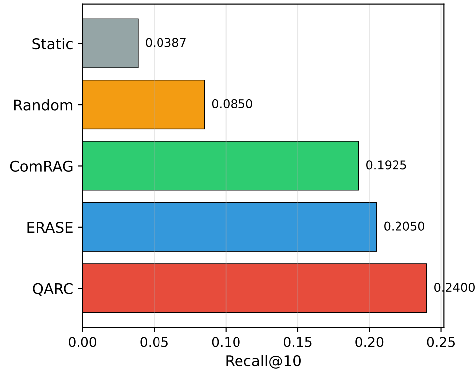
Recall@10
