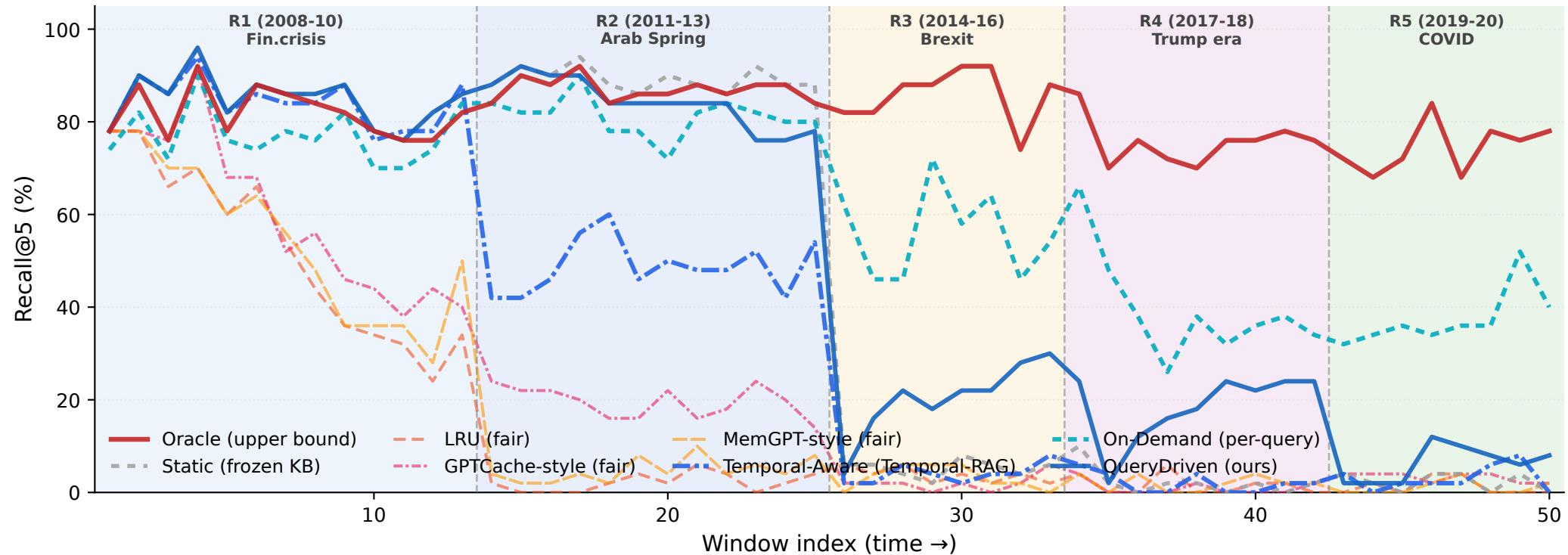
StreamingQA: 14-year real news QA stream (Liška et al., ICML 2022) — 5 year-rounds cold pool=29,819 docs · hot KB=750 slots (40× ratio) | Encoder: BAAI/bge-base-en-v1.5
