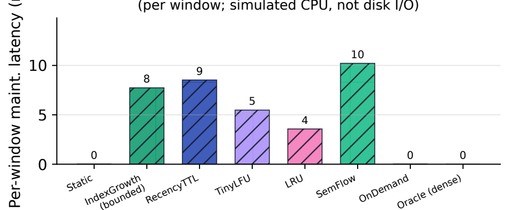
(c) Algorithmic maintenance overhead (per window; simulated CPU, not disk I/O)
