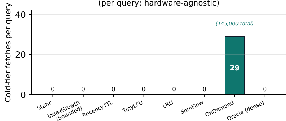
(b) Serve-time cold-tier retrieval cost (per query; hardware-agnostic)
