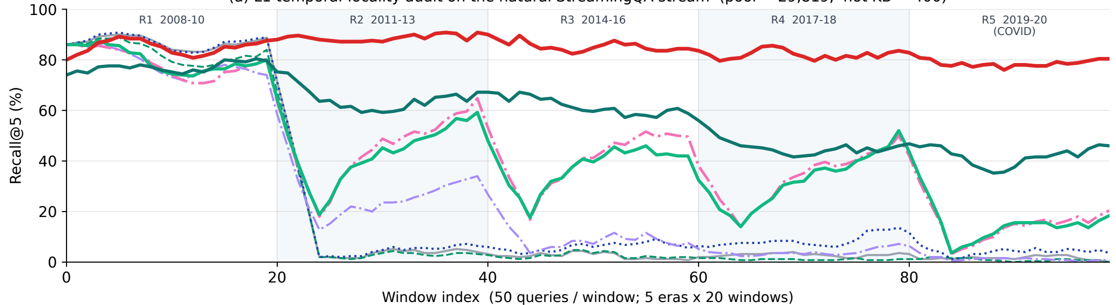
(a) L1 temporal-locality audit on the natural StreamingQA stream (pool = 29,819, hot KB = 400)
