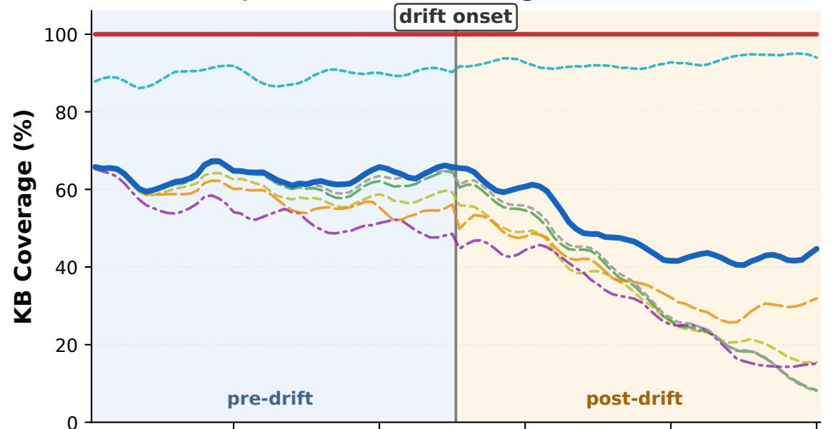
HotpotQA-comparison pool=41,796, KB budget=10,000
