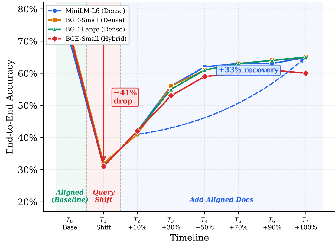
(a) Query Shift → Performance Drop → Recovery
