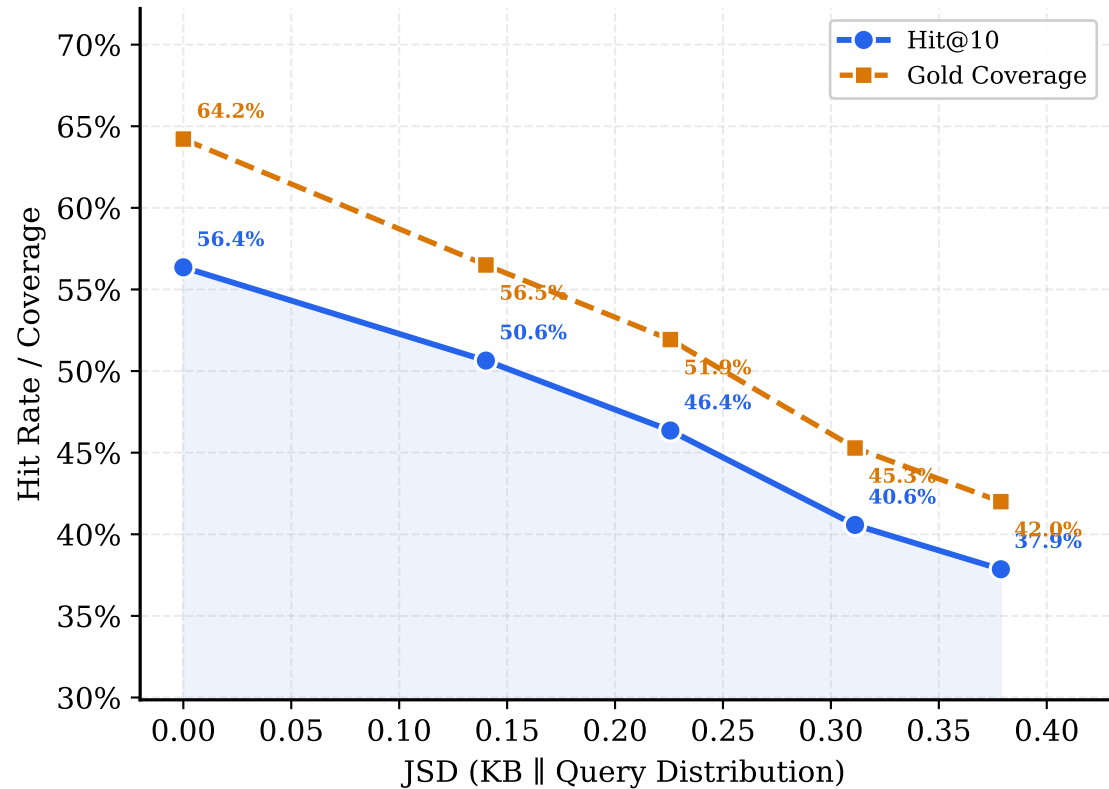
(b) Higher Misalignment → Lower Performance
