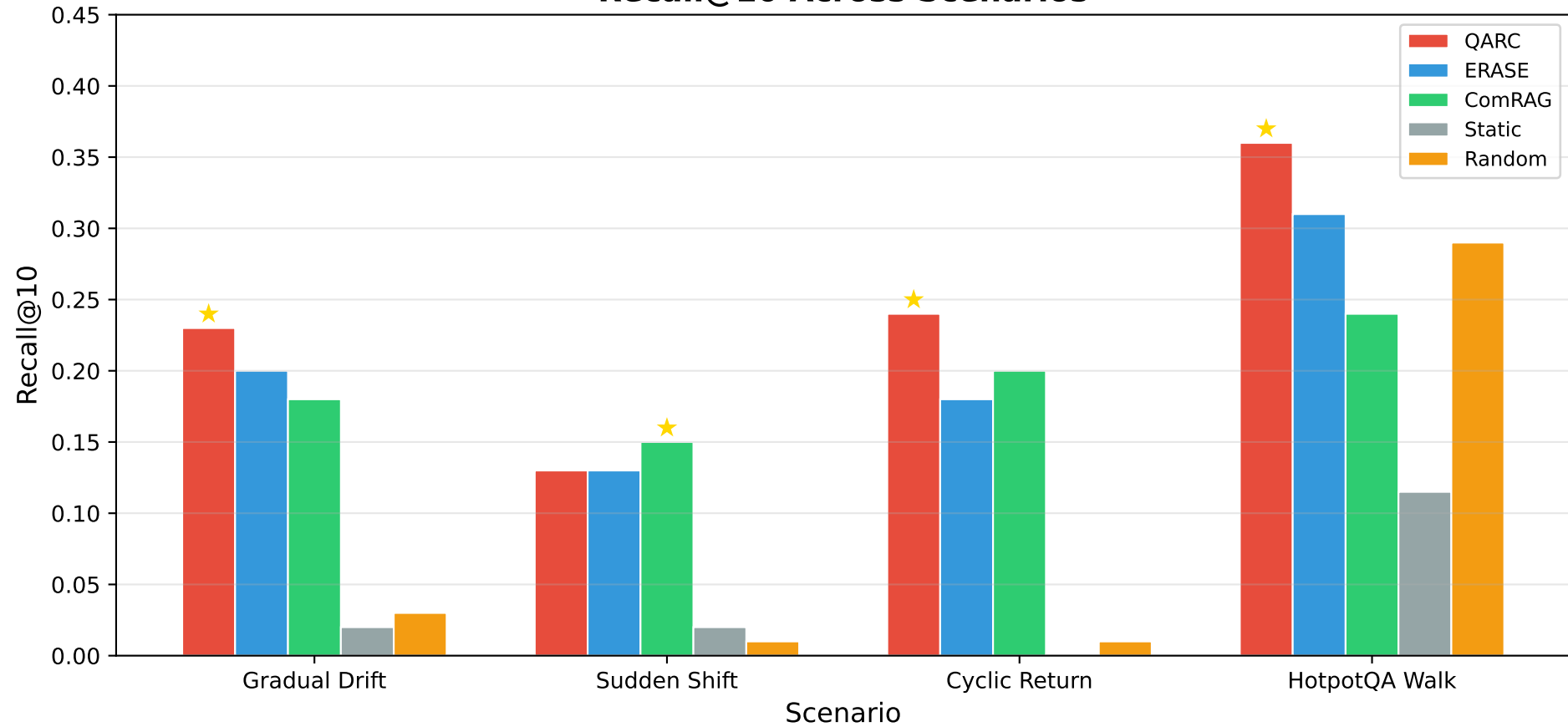
Recall@10 Across Scenarios
