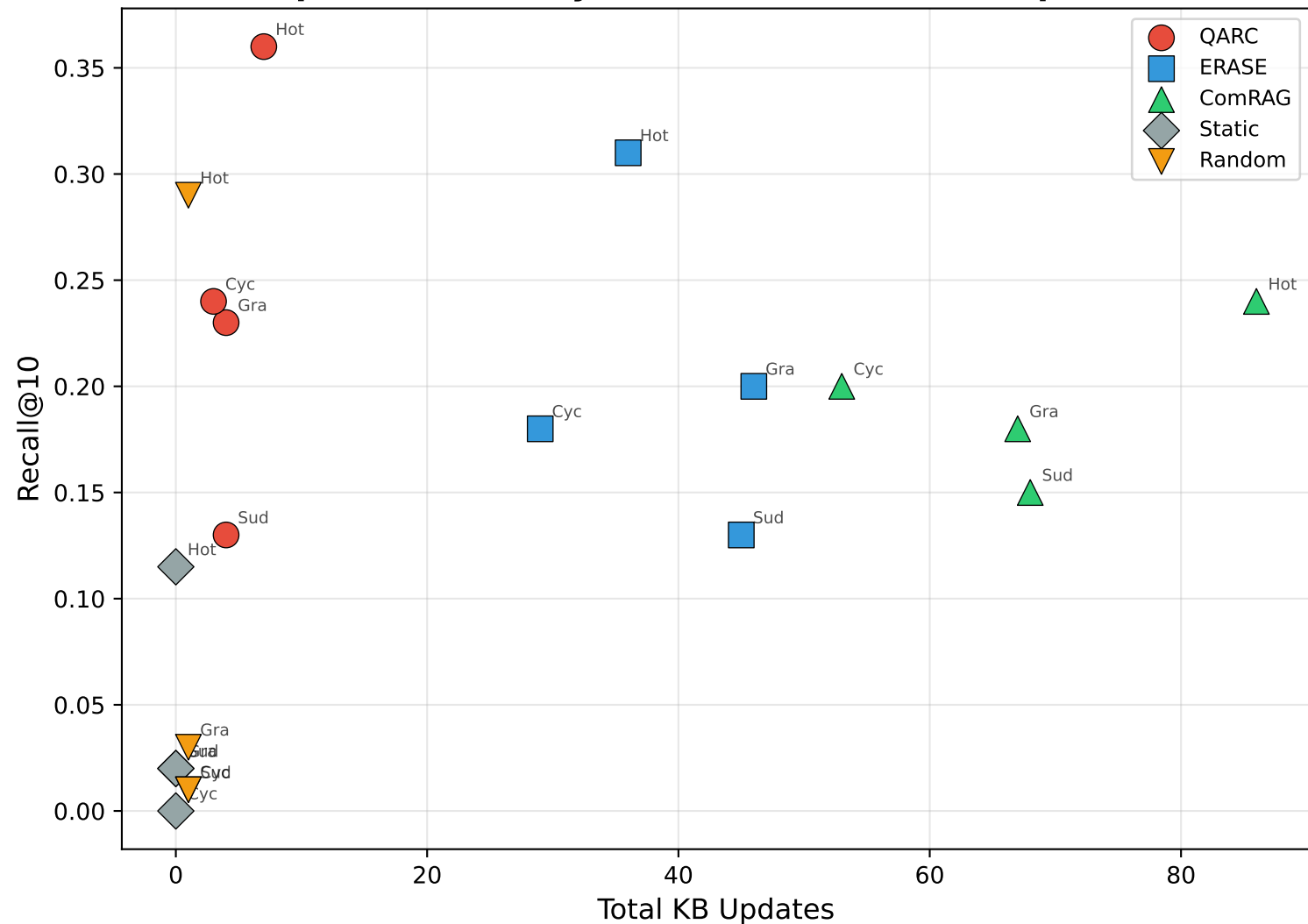
Update Efficiency: Recall vs. Number of Updates
