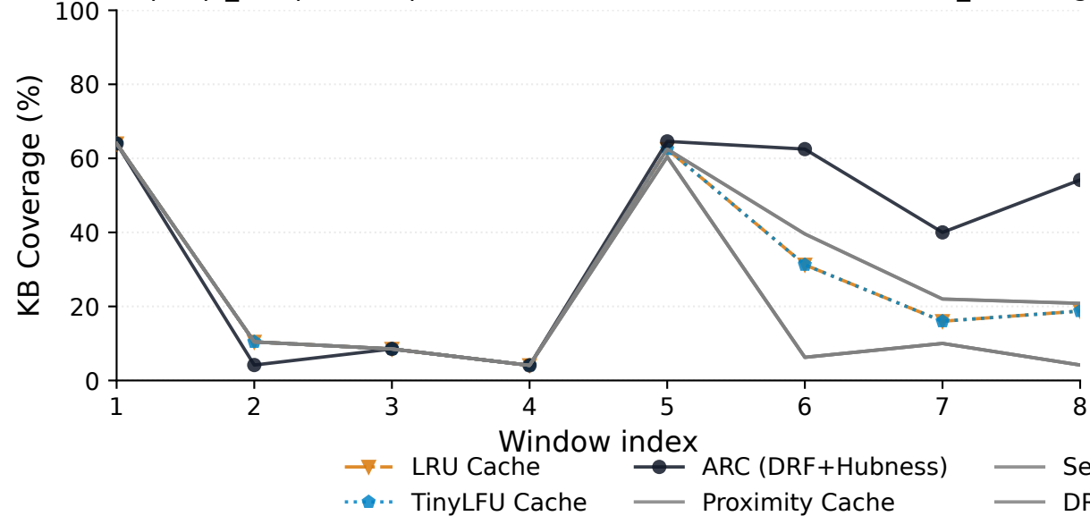
hotpotqa_comparison pool=30,280 KB=3,028 8x25 factorized_recurring
