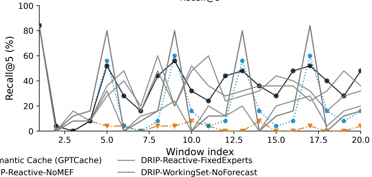
Recall@5
