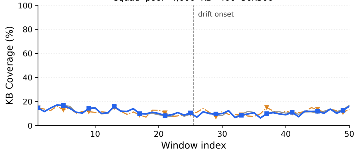
squad pool=4,000 KB=400 50x300
