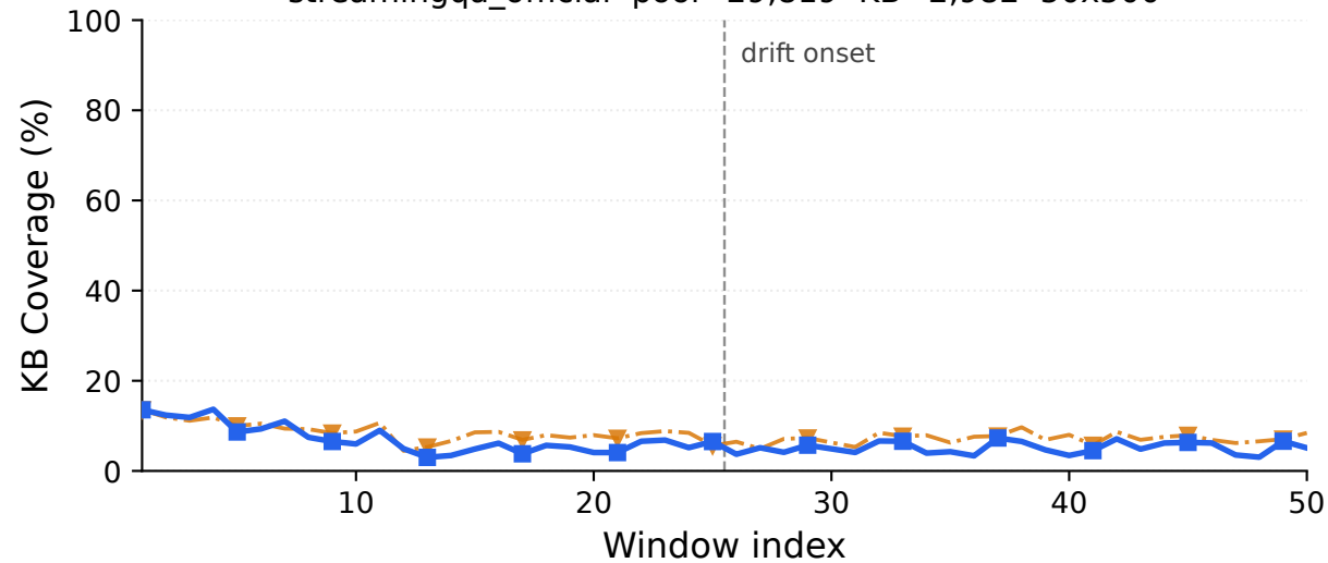
streamingqa_official pool=29,819 KB=2,982 50x500
