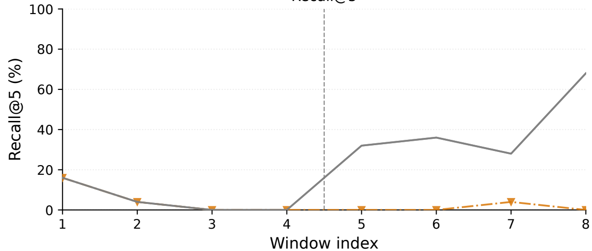
Recall@5
