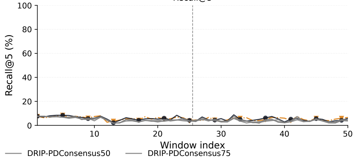
Recall@5
