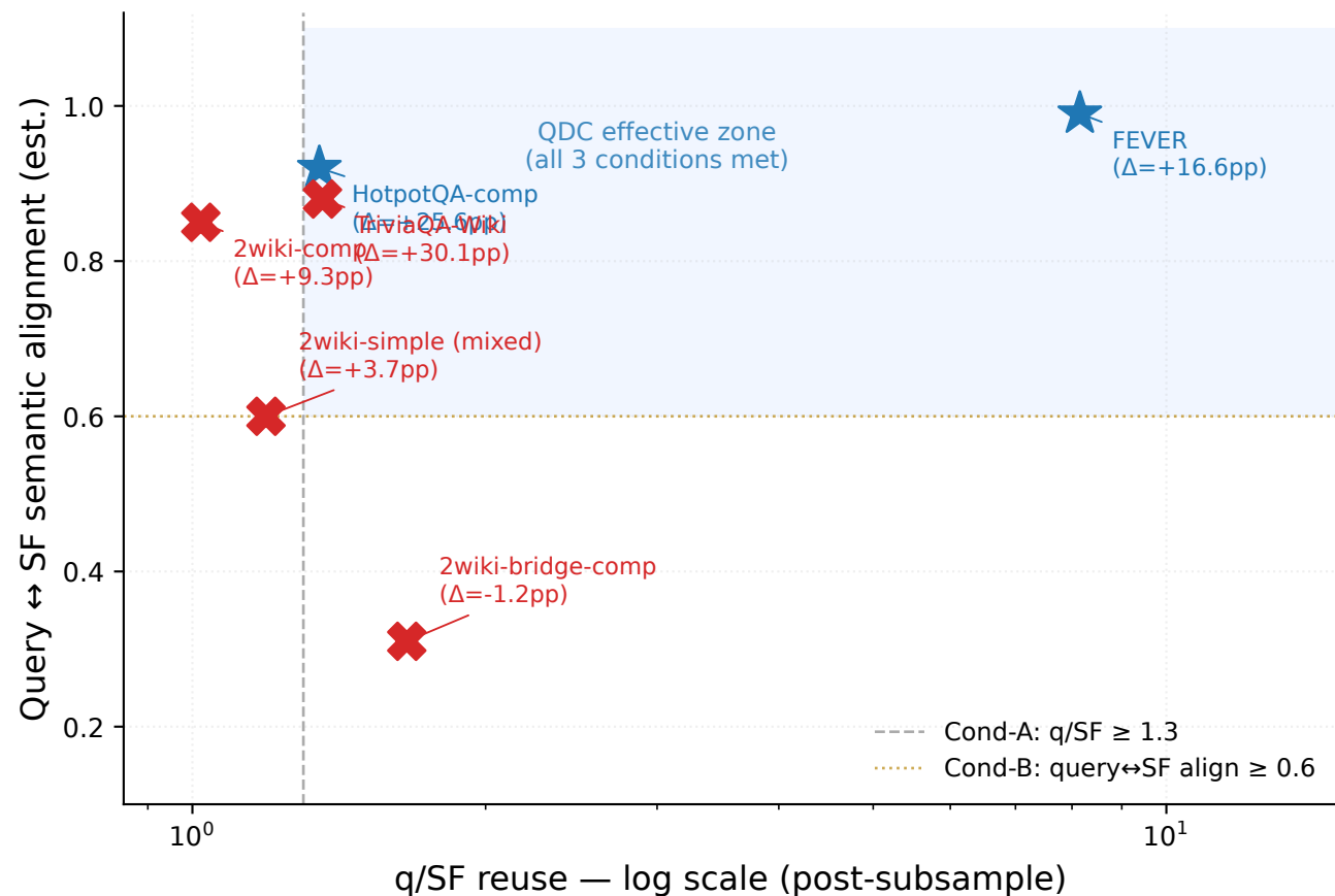
QDC Condition Space (★ = all conditions met, ✕ = at least one fails)
