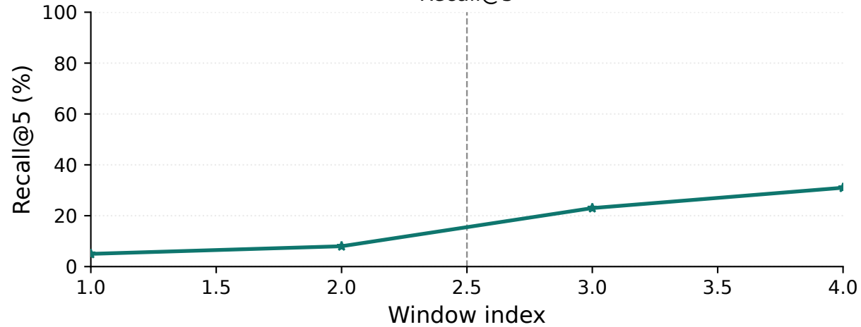
Recall@5
