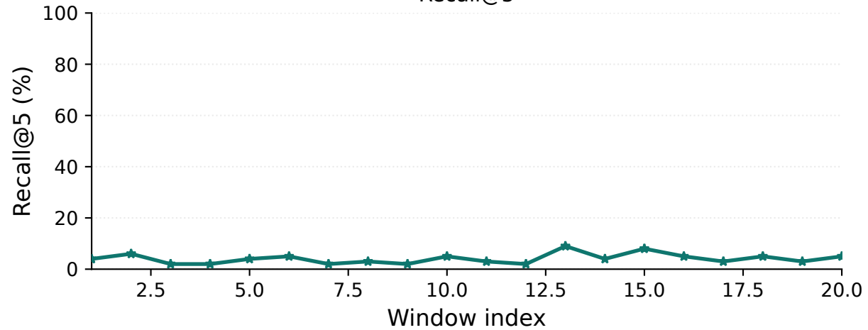
Recall@5
