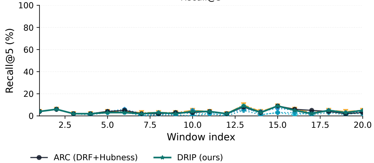
Recall@5
