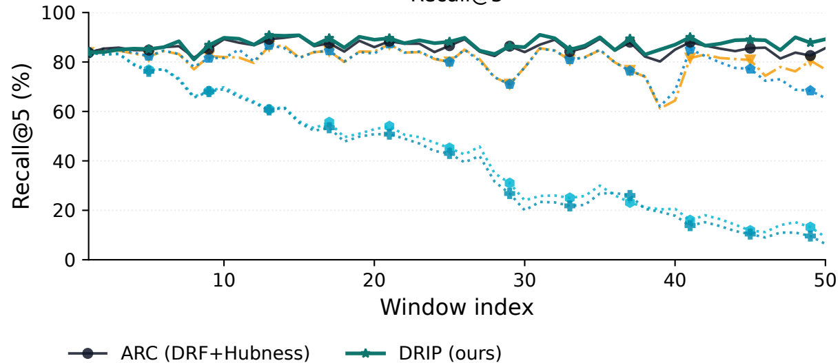
Recall@5
