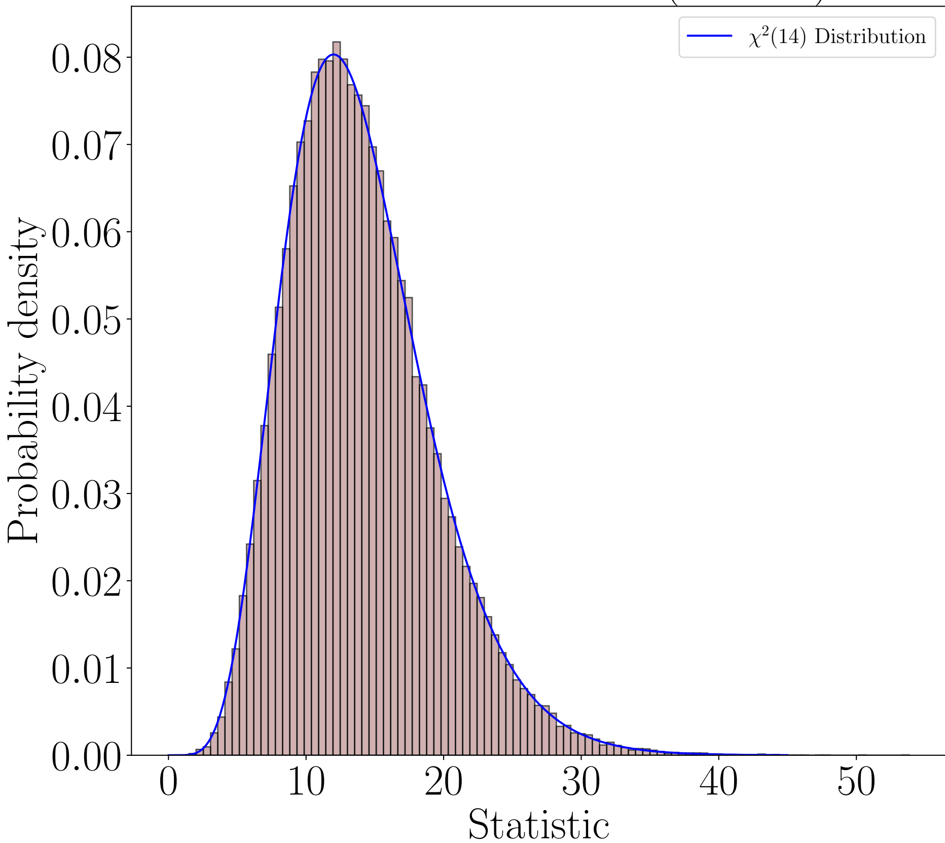
Distribution of statistic ( K = 15 )
