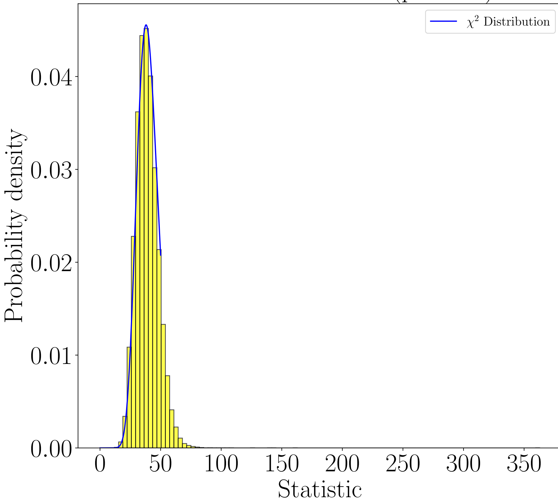
Distribution of statistic (pairwise)
