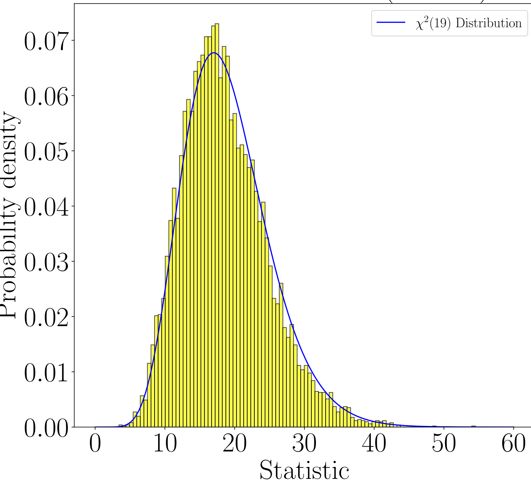
Distribution of statistic ( K = 20 )
