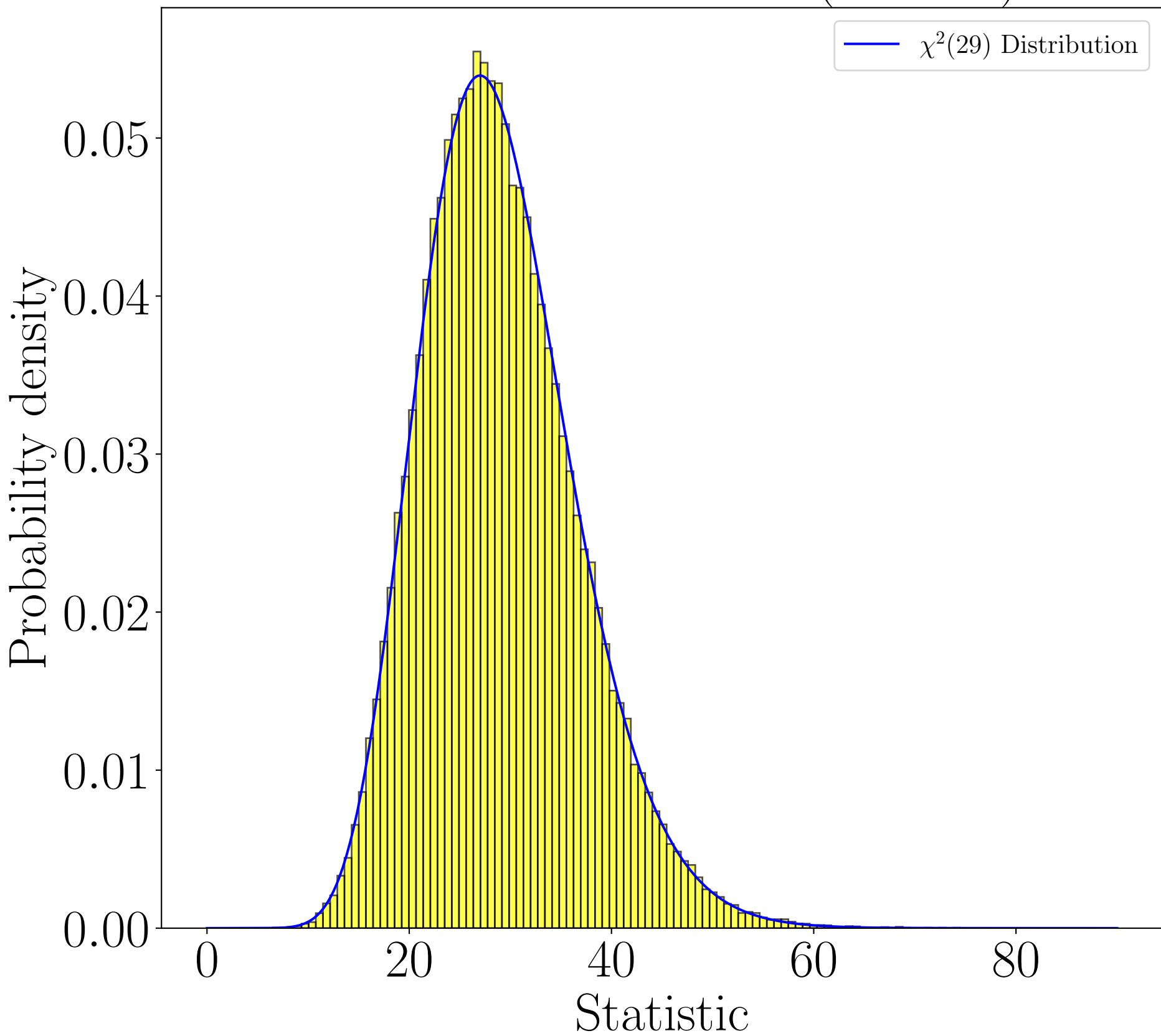
Distribution of statistic ( K = 30 )
