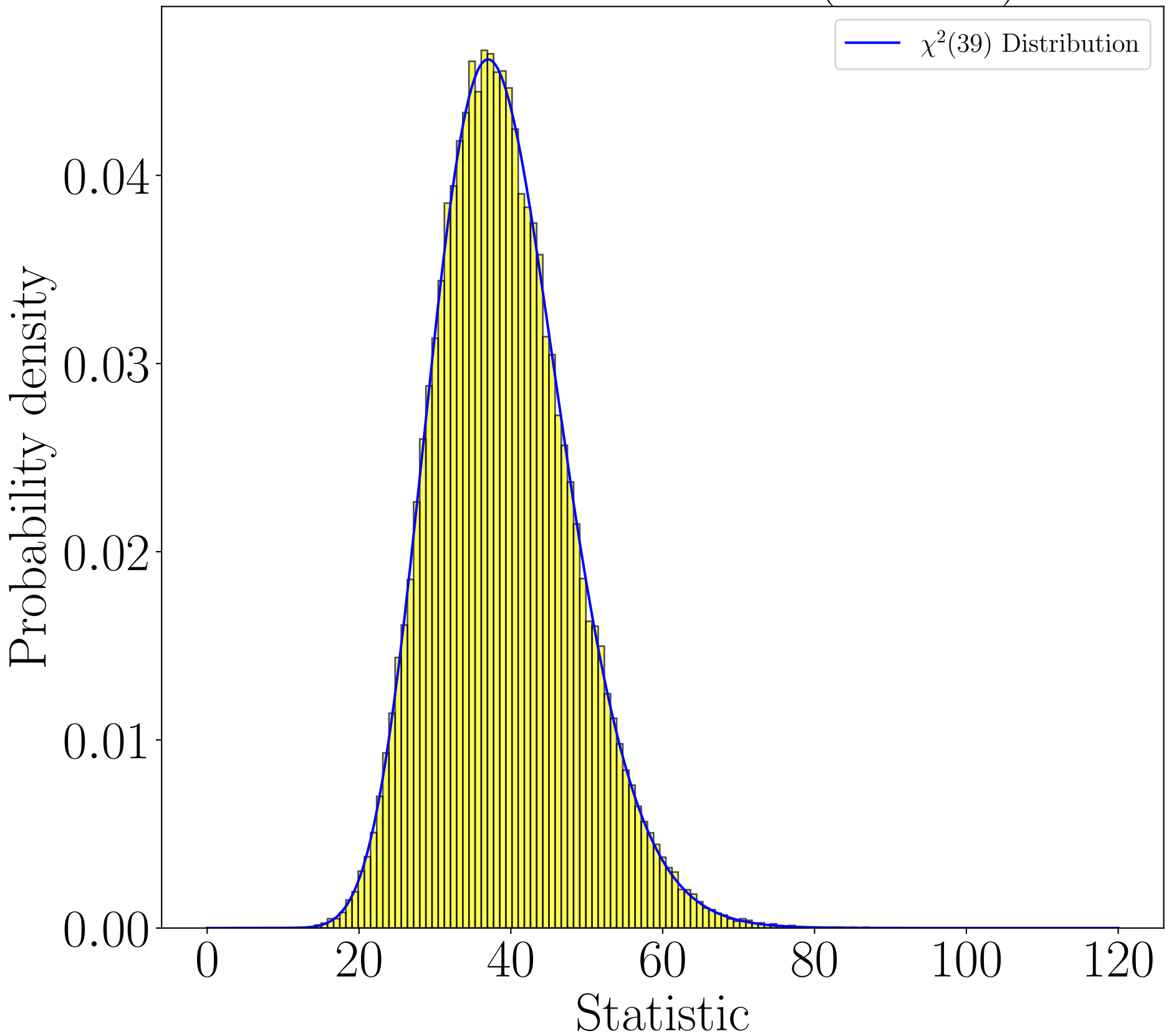
Distribution of statistic ( K = 40 )
