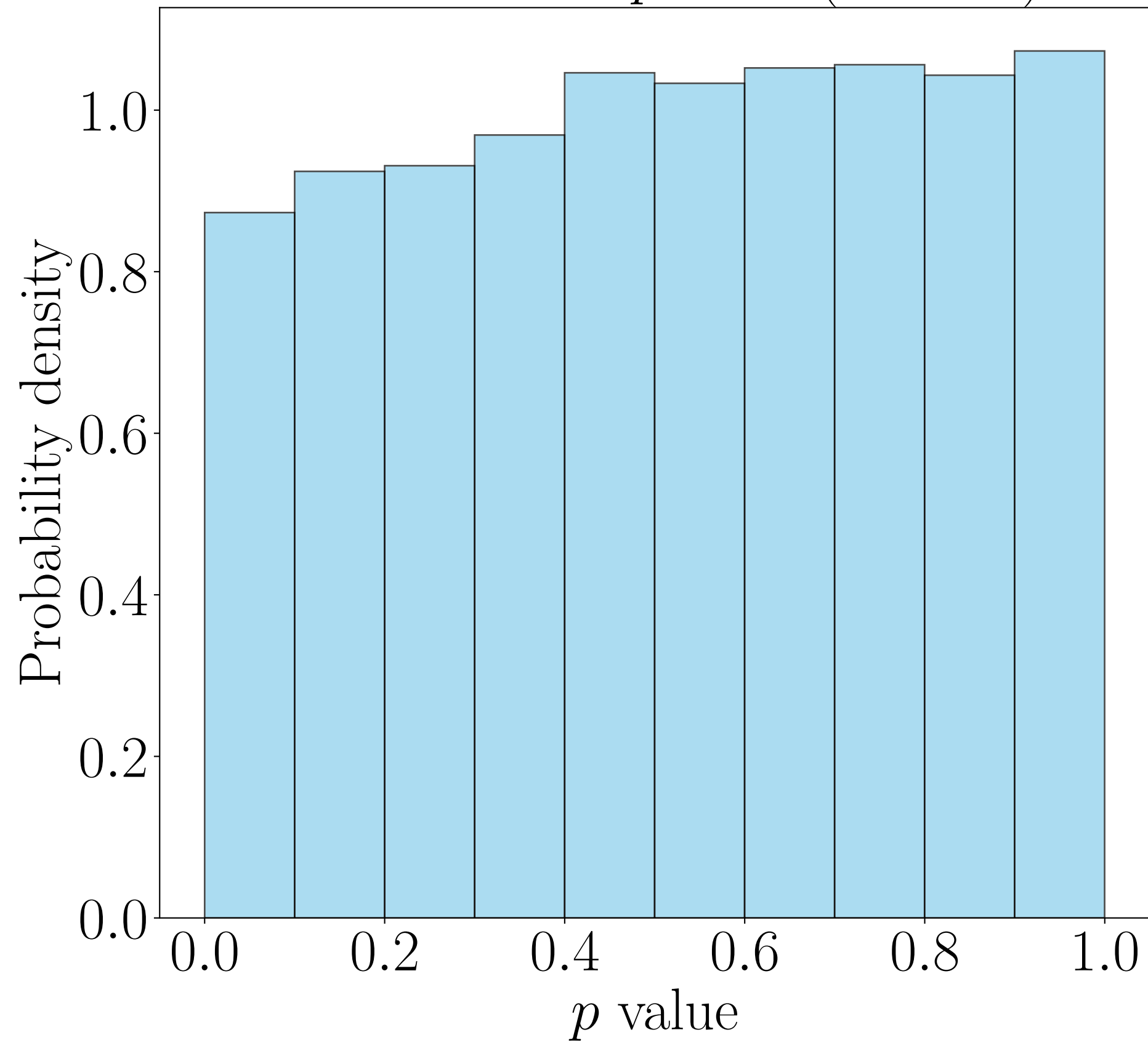
Distribution of p value ( K = 20 )
