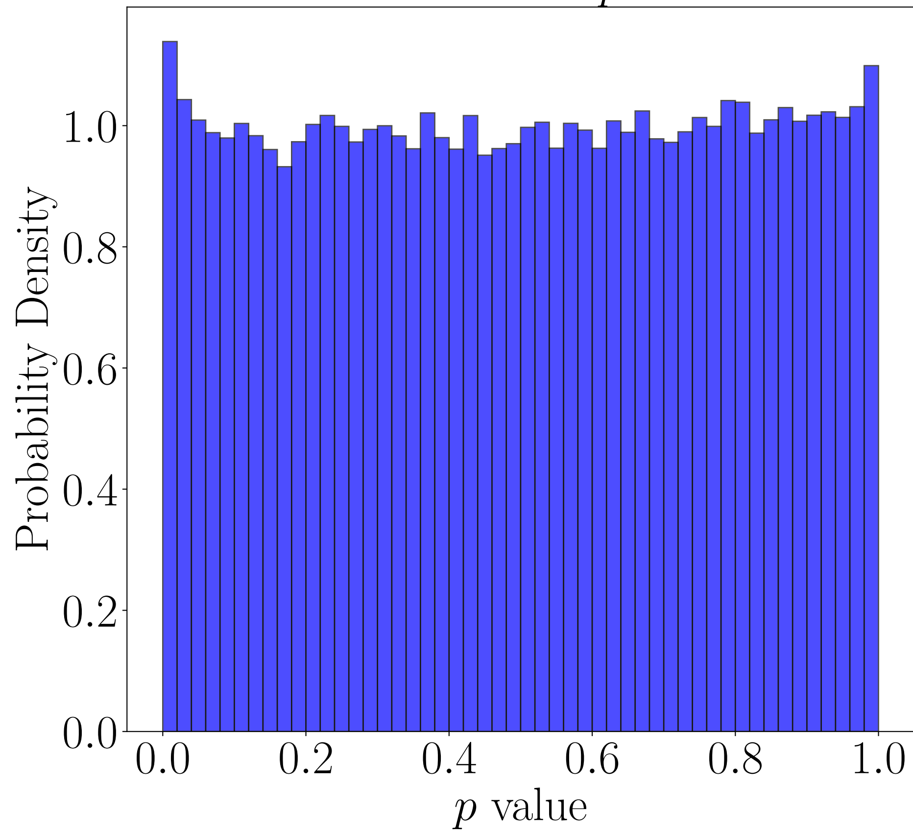
Distribution of p value
