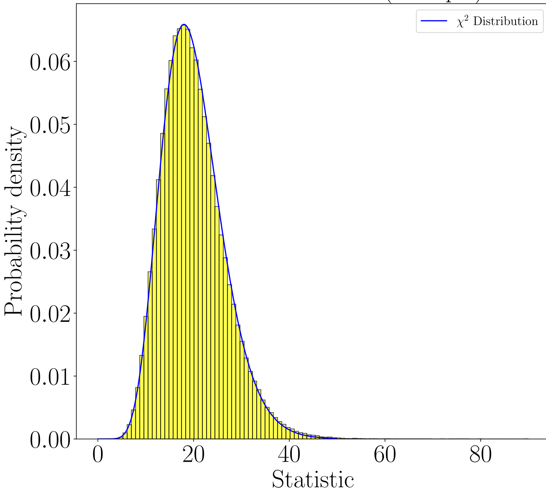
Distribution of statistic (multiple)
