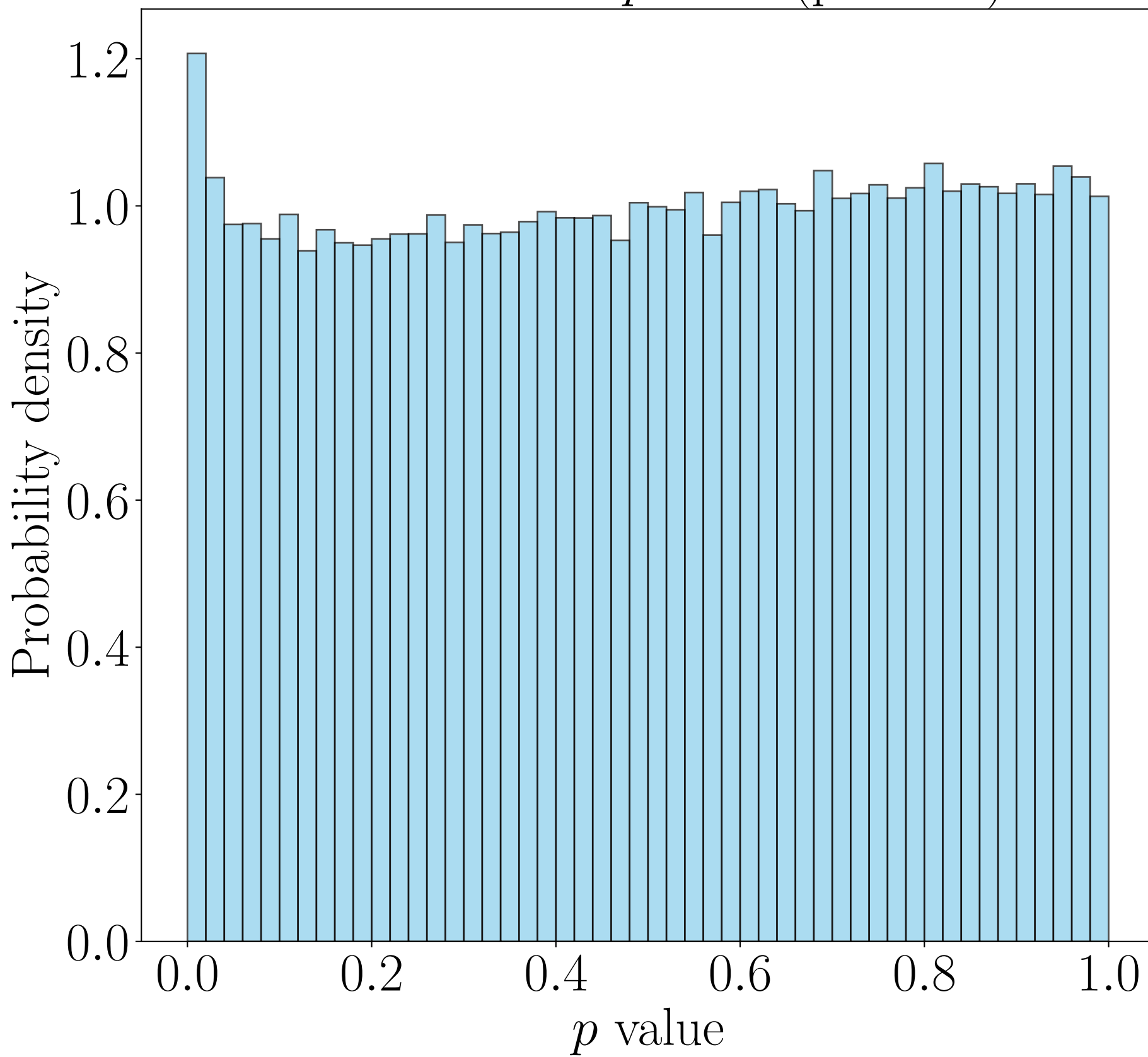
Distribution of p value (pairwise)
