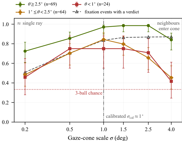
Top-1 binding accuracy
