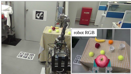
(e) Selecting and grasping the same pink apple
