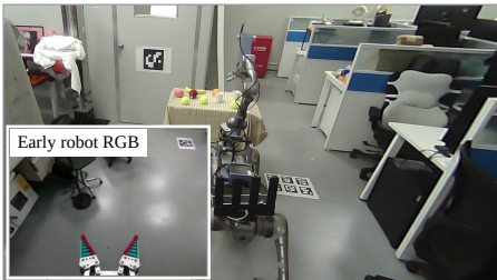
(d) Approaching the mapped target Target unseen in the early robot view
